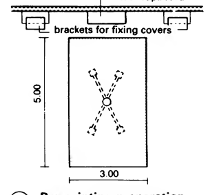
⑥ Pre-painting preparation area - with or without lifting frame 3.0m x 5.0m
